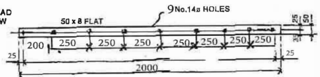
LOWER CAGE STRAP REF. AX12
