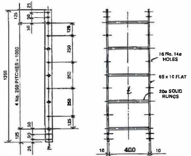
SHORT LADDER SECTION REF AX2
