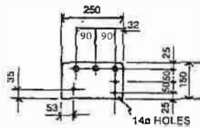
TOP STEP DETAIL REF. AX5 (ITEM AX10 REQUIRED TO FIX TO AX1 OR 2)
