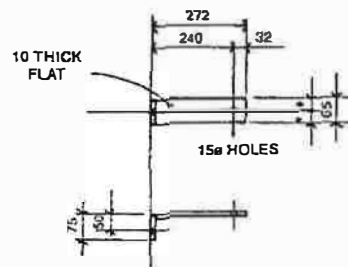
LADDER STAY REF. AX7 (SOLD IN PAIRS)
