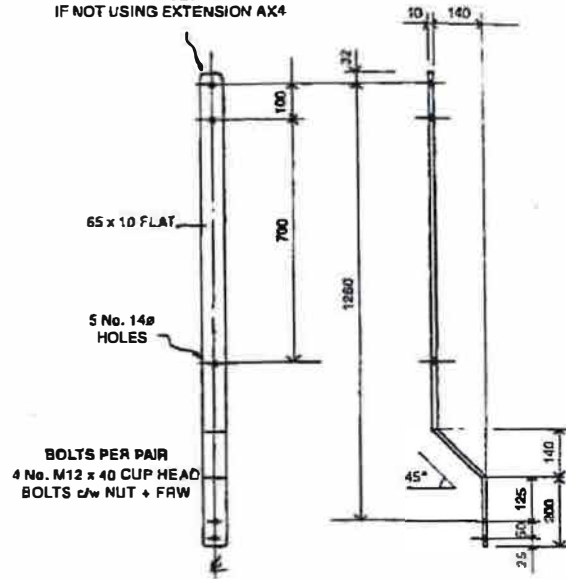
LADDER EXTENSION REF AX3 (SOLD IN PAIRS)
