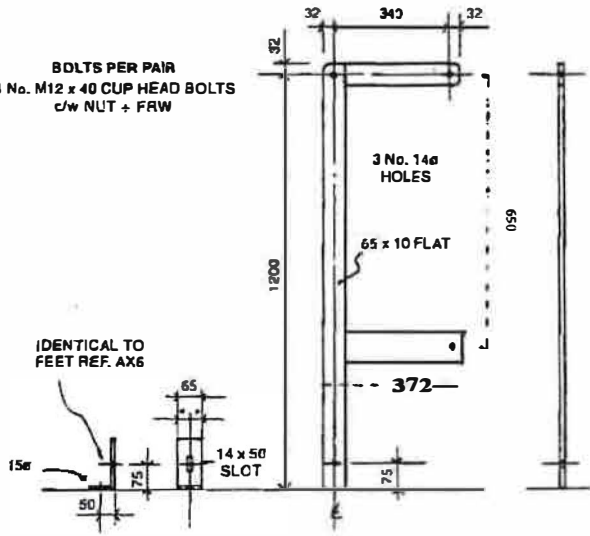
EXTENSION TO FLOOR REF AX4 (SOLD IN PAIRS)
