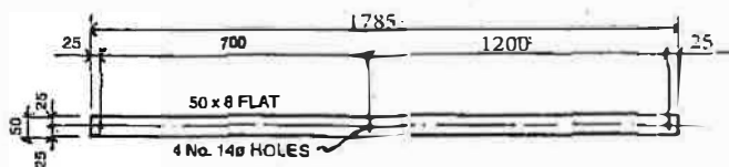
TOP CAGE STRAP REF. AX11
