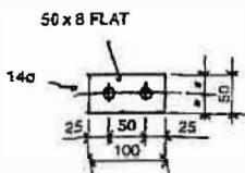
CAGE SPLICE REF. AX13
