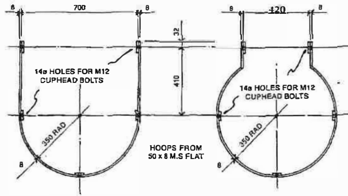
TOP HOOPS REF. AX8
