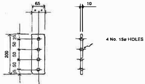
SPLICE PLATES REF. AX10 (SOLD IN PAIRS)
