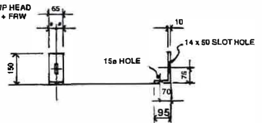
LADDER FEET REF AX6 (SOLD IN PAIRS)
